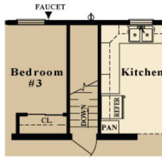
OPT. BASEMENT STAIRWELL LAYOUT
