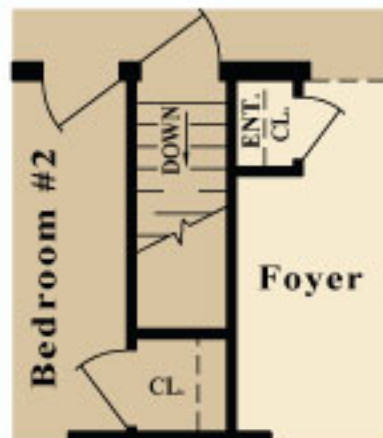
OPT. BASEMENT STAIRWELL LAYOUT
